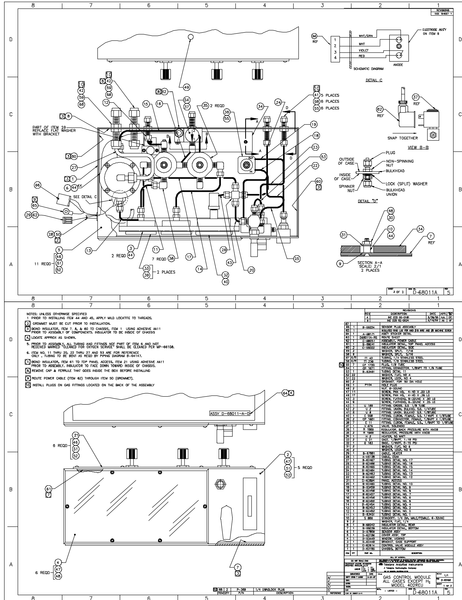
Title: G:\MASTER\68000\D68011A-5.DWG
