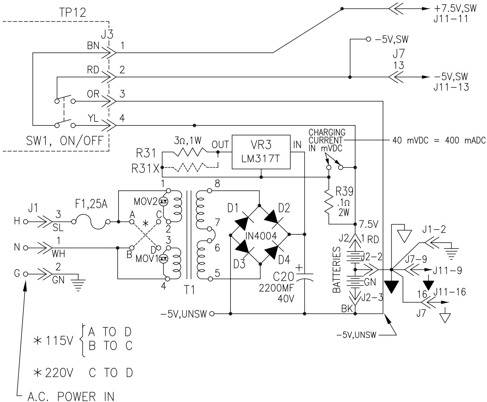
MAX5 POWER SUPPLY/CHARGER SCHEMATIC
