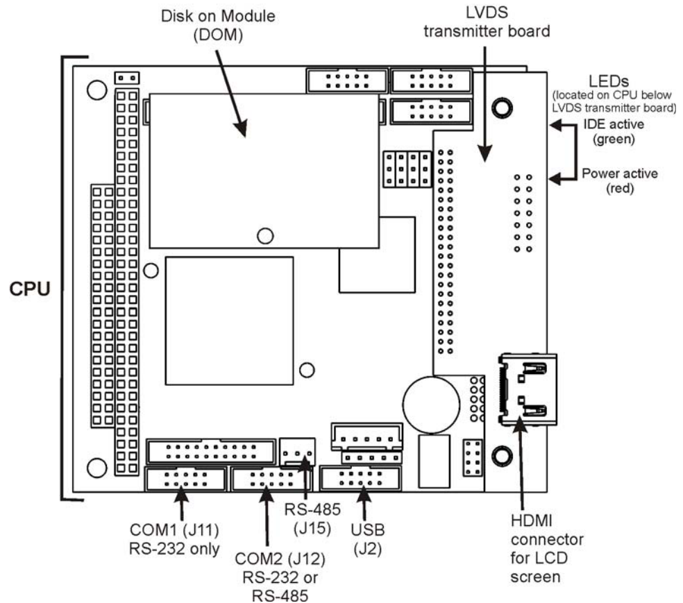
Figure 13-14: CPU Board
