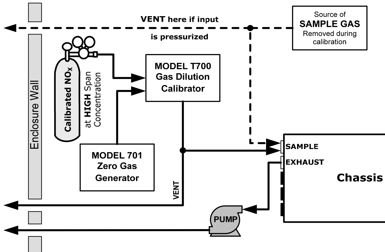
Figure 3-17: Gas Line Connections from Calibrator – Basic 9110T Configuration
