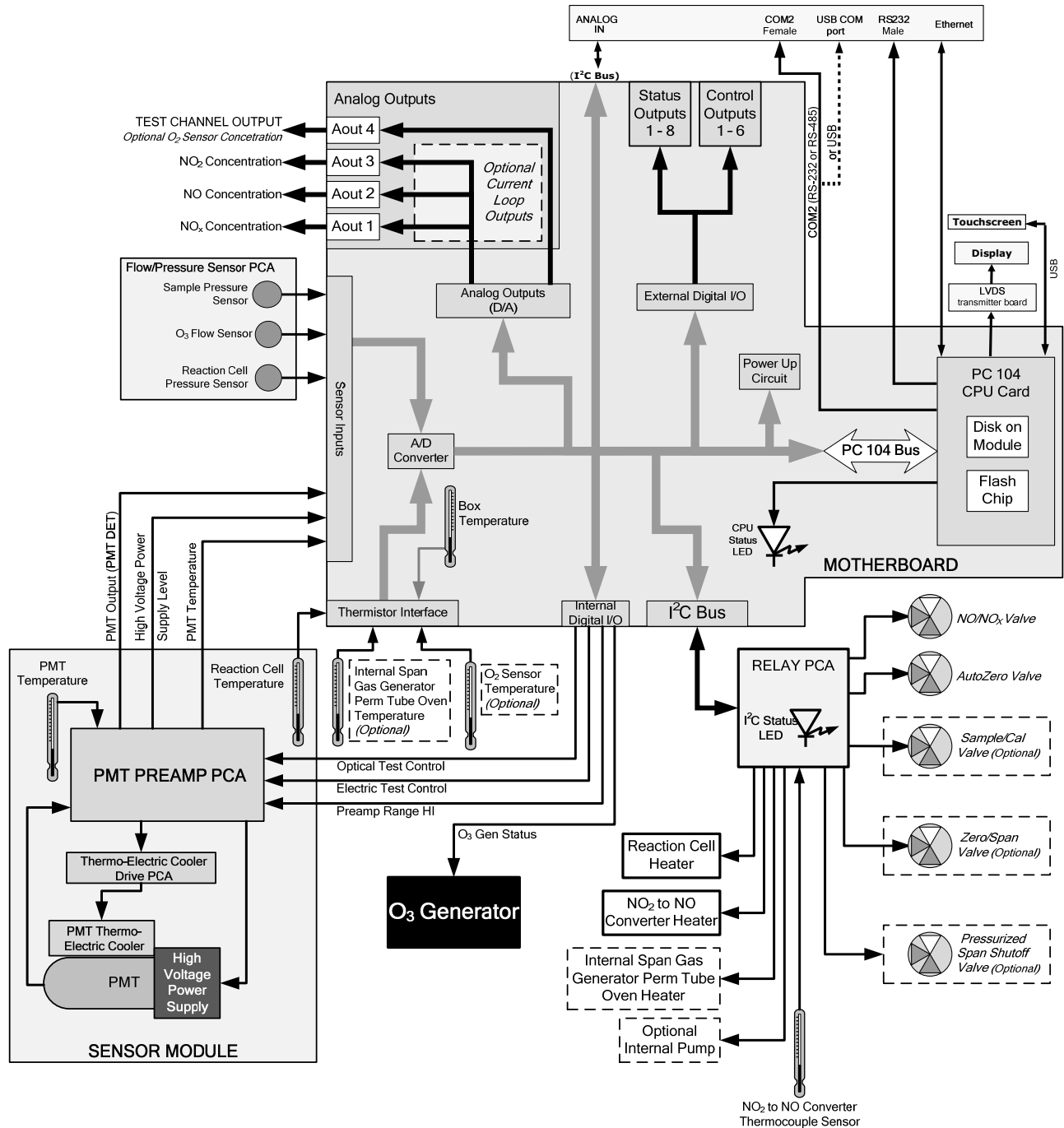
Figure 13-13: 9110T Electronic Block Diagram
