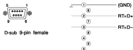
< RS-485 connector >
